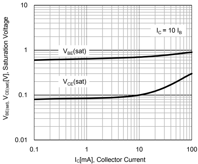
Fig.3 Base-Emitter Saturation Voltage VS. Collector-Emittor Saturation
